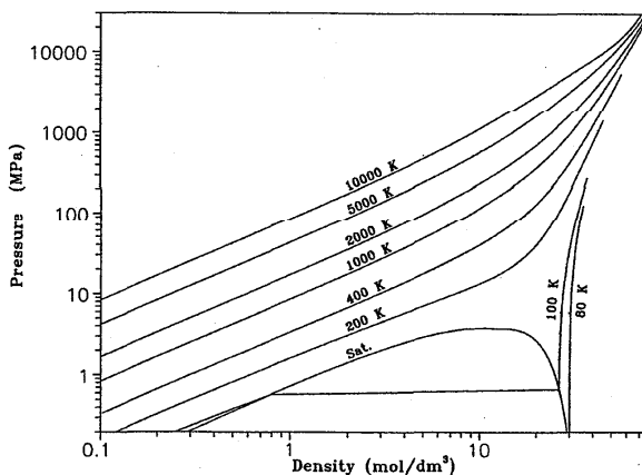
FIG. 27. Pressure versus density diagram for air.
