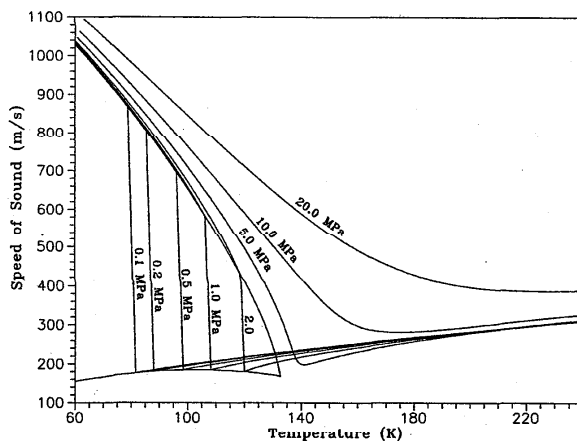
FIG. 26. Speed of sound versus temperature diagram for air.
