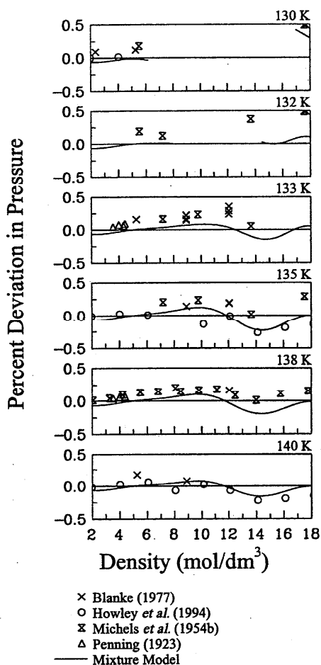
FIG. 11. Comparisons of pressures calculated with the equation of state to experimental data for air in the critical region.
