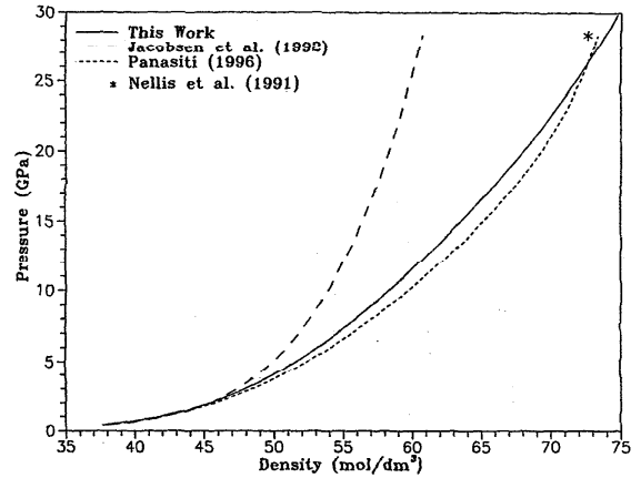
FIG. 7. Calculated Hugoniot curve for air.
