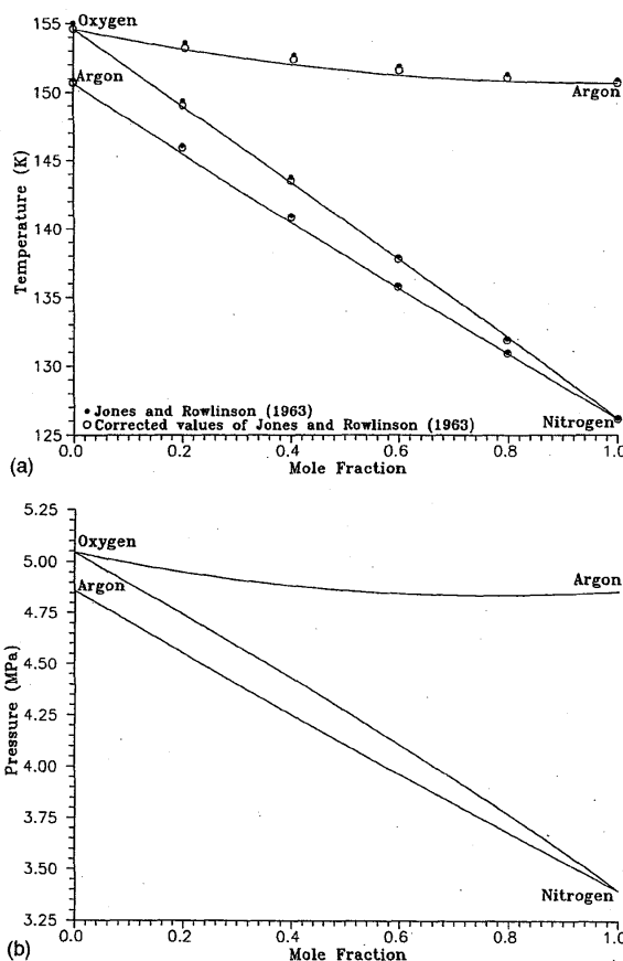
Fig. 8. Critical lines for nitrogen-argon, nitrogen-oxygen, and argon-oxygen binary mixtures.
