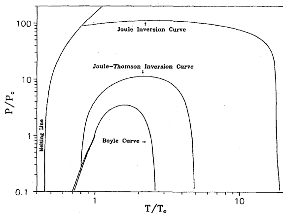
Fig. 28. Characteristic curves for air.
